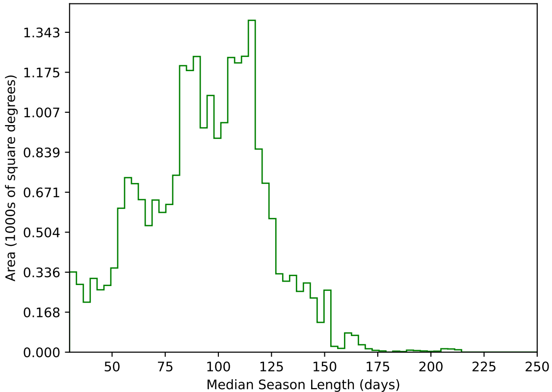
too_elab_r32_d3_gz_v3.4_10yrs All sky g band: Median Season Length
