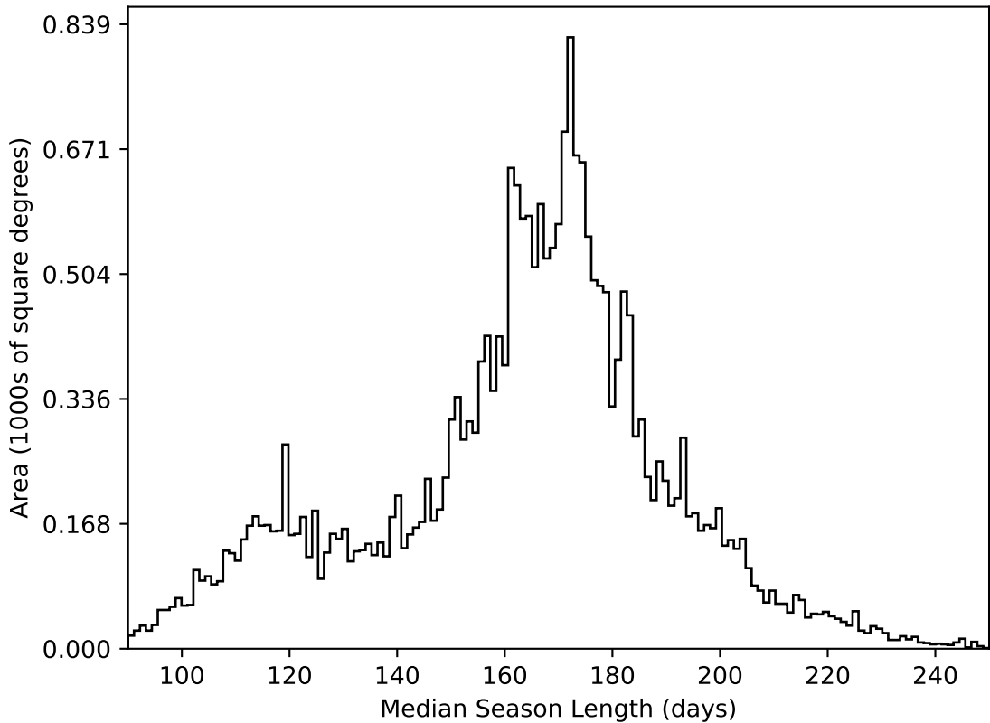
too_elab_r32_d3_gz_v3.4_10yrs All sky all bands: Median Season Length
