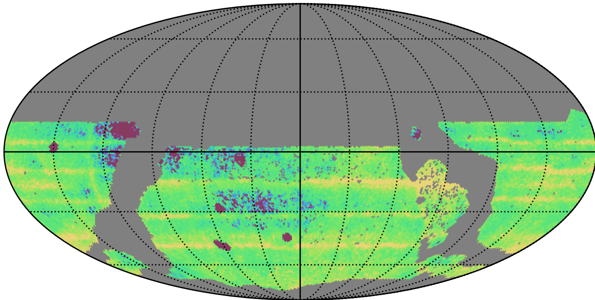
too_elab_r32_d3_gz_v3.4_10yrs WFD: Median Intra-Night Gap
