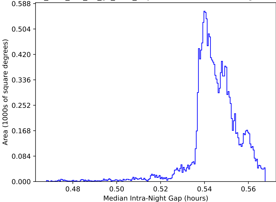
too_elab_r32_d3_gz_v3.4_10yrs WFD: Median Intra-Night Gap
