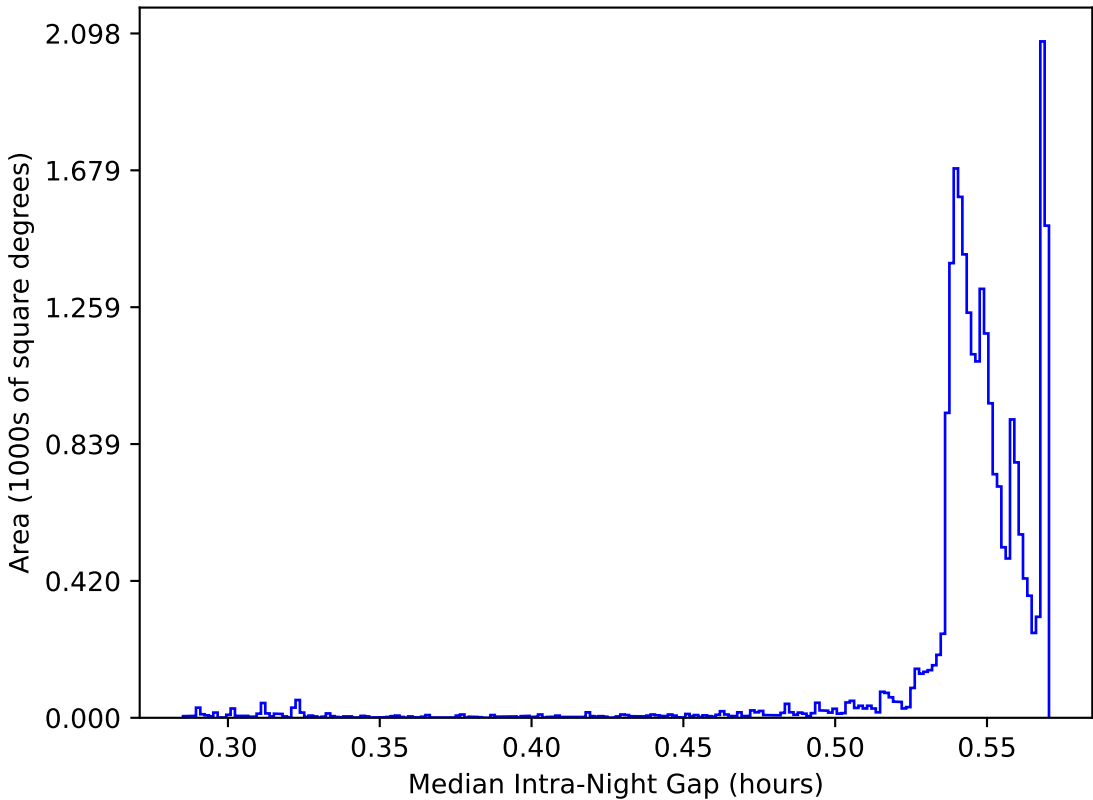
too_elab_r32_d3_gz_v3.4_10yrs All sky: Median Intra-Night Gap
