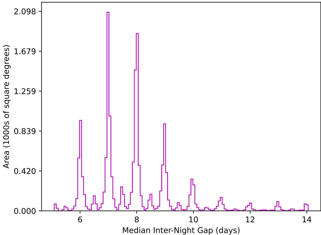
too_elab_r32_d3_gz_v3.4_10yrs WFD z band: Median Inter-Night Gap
