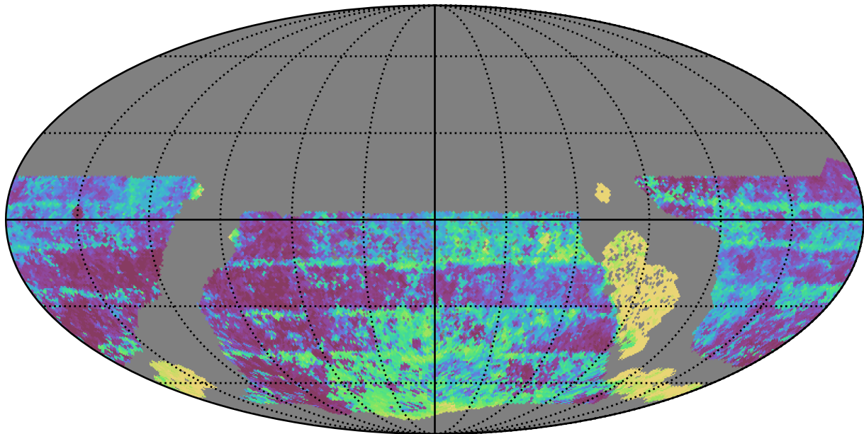
too_elab_r32_d3_gz_v3.4_10yrs WFD y band: Median Inter-Night Gap
