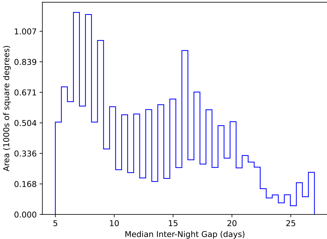
too_elab_r32_d3_gz_v3.4_10yrs WFD y band: Median Inter-Night Gap
