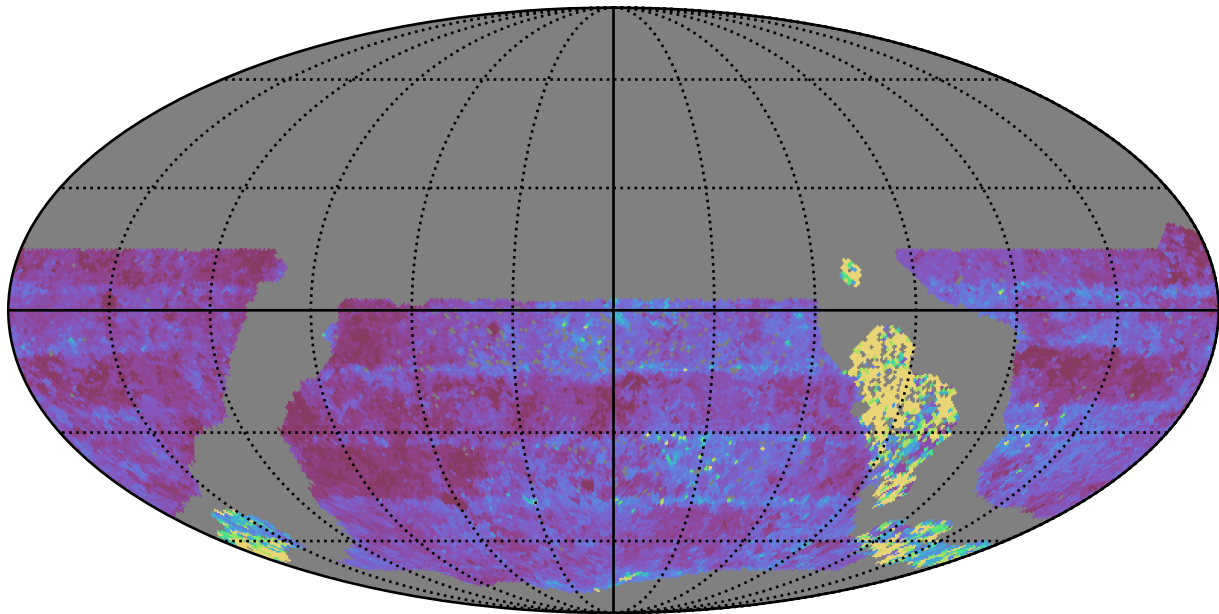
too_elab_r32_d3_gz_v3.4_10yrs WFD u band: Median Inter-Night Gap
