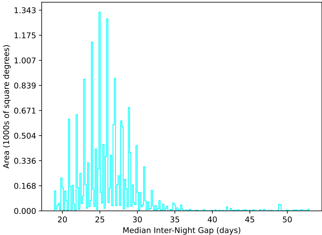
too_elab_r32_d3_gz_v3.4_10yrs WFD u band: Median Inter-Night Gap
