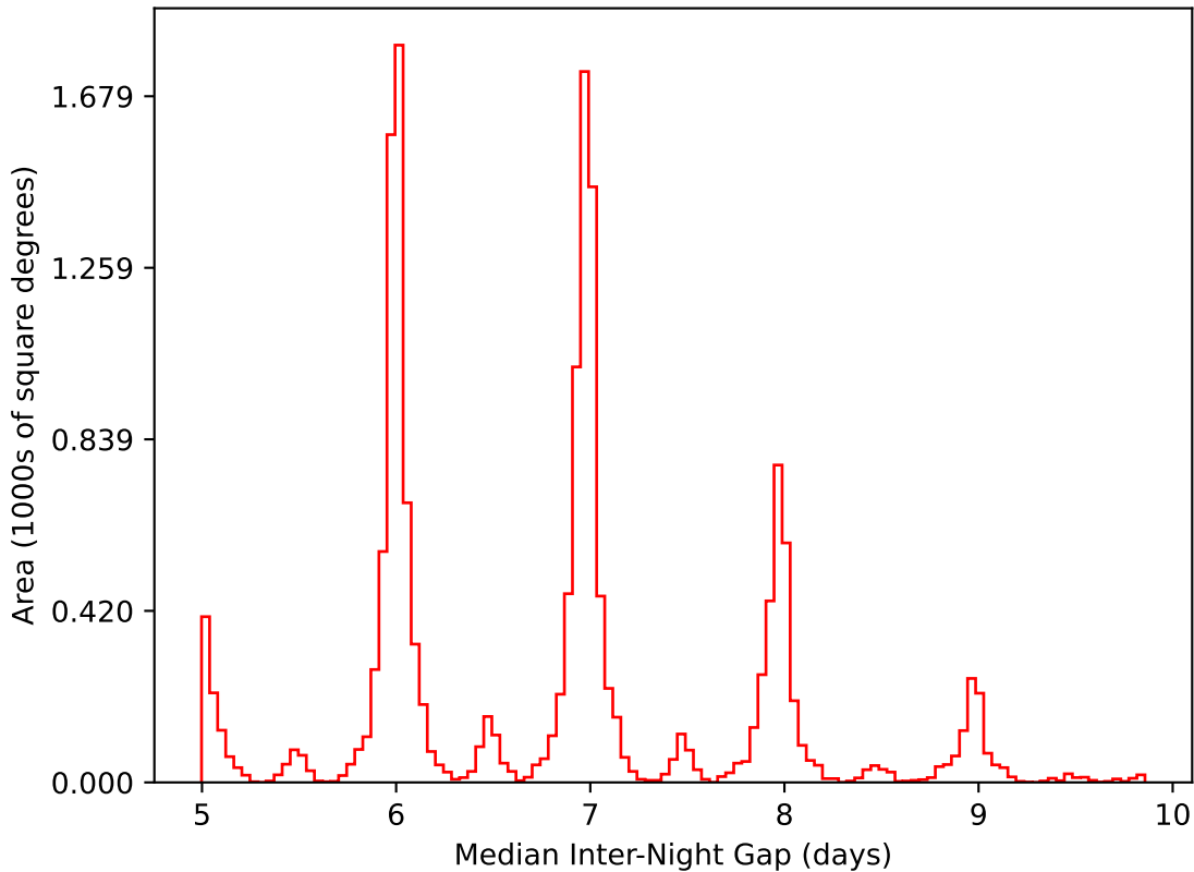
too_elab_r32_d3_gz_v3.4_10yrs WFD i band: Median Inter-Night Gap
