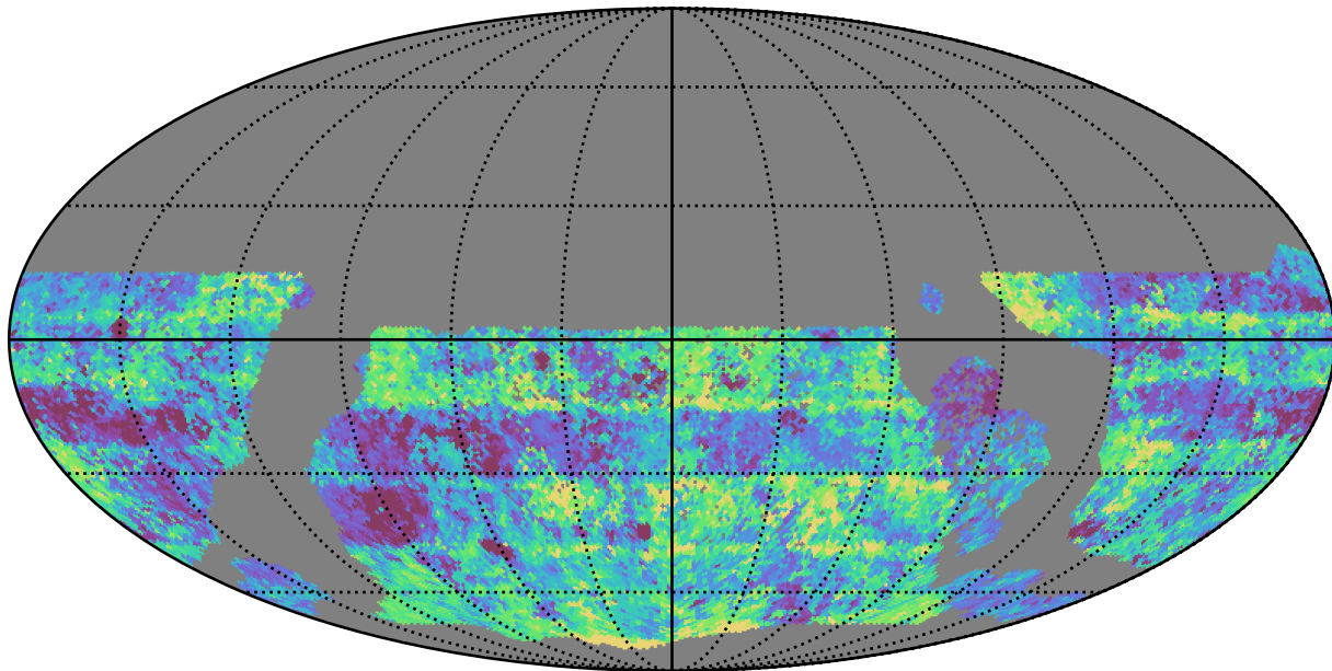
too_elab_r32_d3_gz_v3.4_10yrs WFD g band: Median Inter-Night Gap
