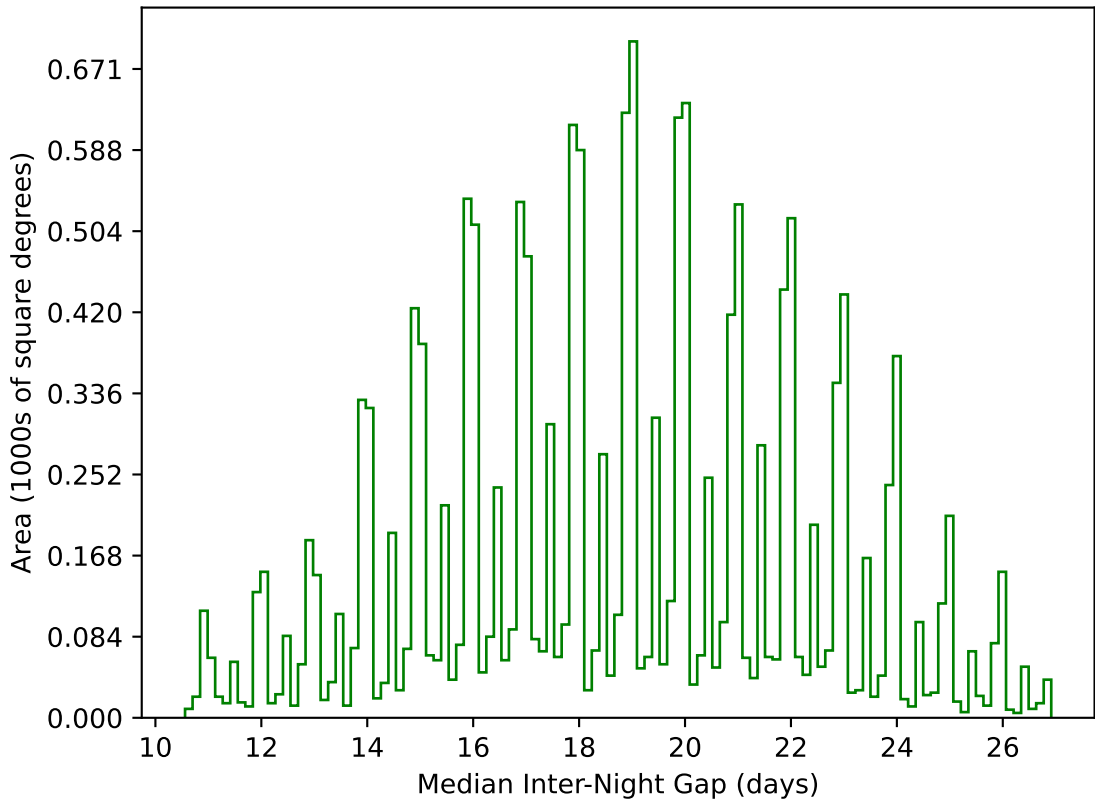
too_elab_r32_d3_gz_v3.4_10yrs WFD g band: Median Inter-Night Gap
