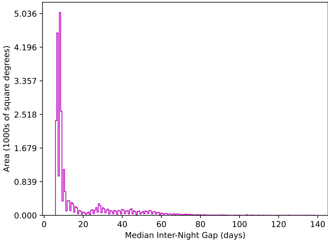
too_elab_r32_d3_gz_v3.4_10yrs All sky z band: Median Inter-Night Gap
