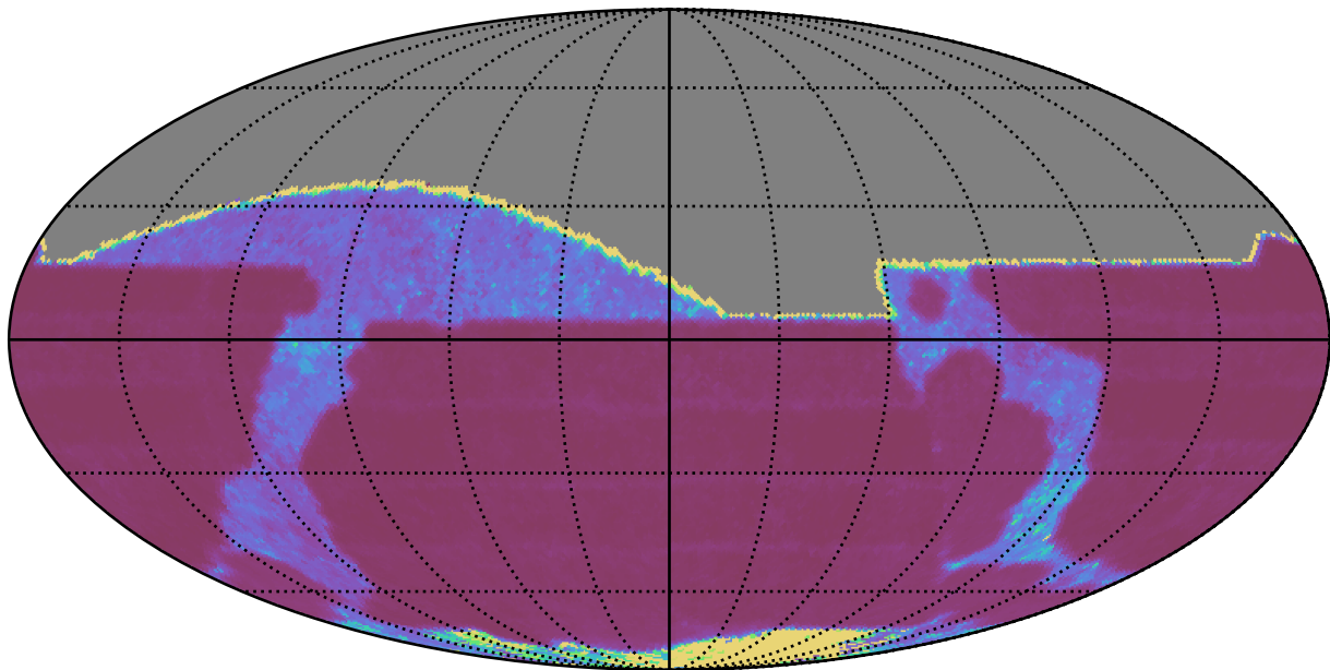
too_elab_r32_d3_gz_v3.4_10yrs All sky r band: Median Inter-Night Gap
