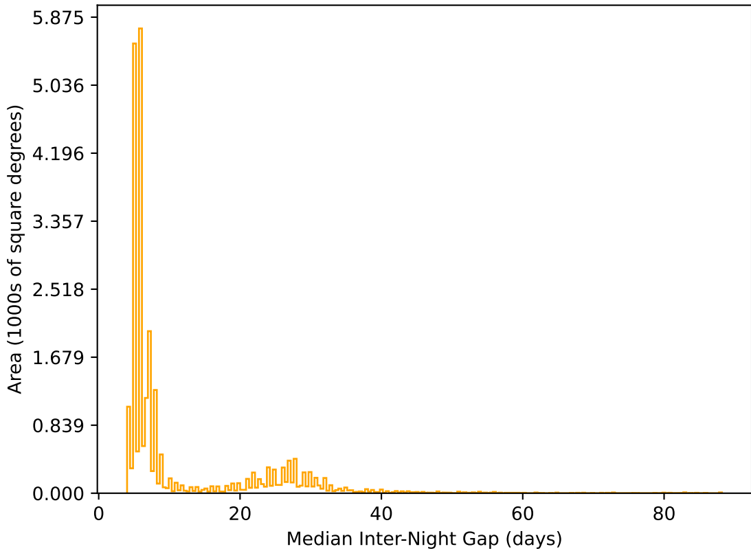
too_elab_r32_d3_gz_v3.4_10yrs All sky r band: Median Inter-Night Gap
