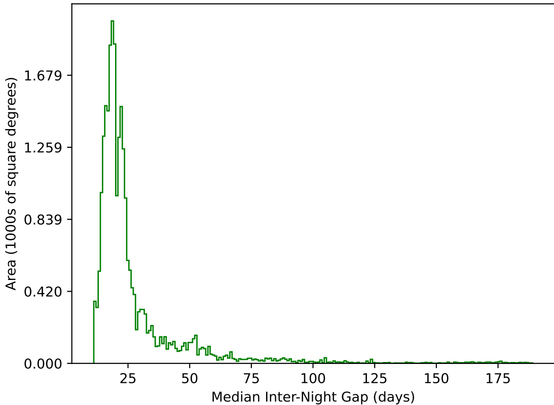
too_elab_r32_d3_gz_v3.4_10yrs All sky g band: Median Inter-Night Gap
