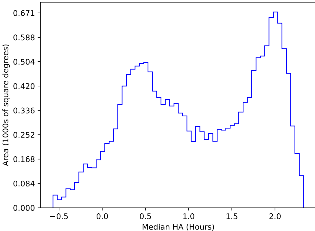
too_elab_r32_d3_gz_v3.4_10yrs WFD z band: Median HA
