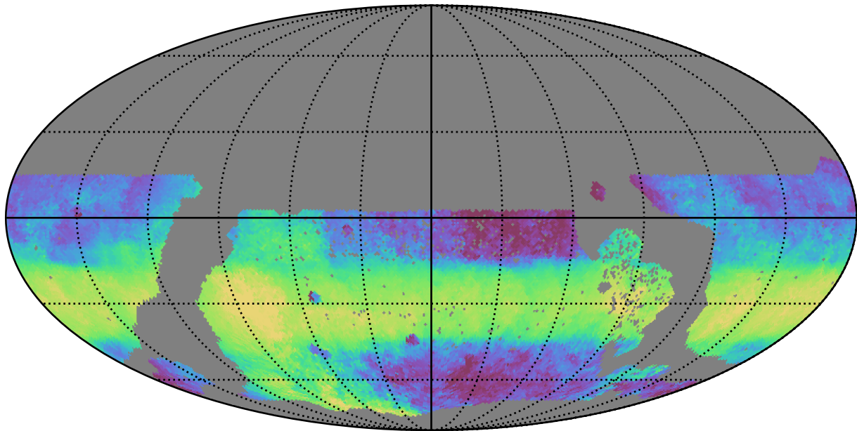
too_elab_r32_d3_gz_v3.4_10yrs WFD y band: Median HA
