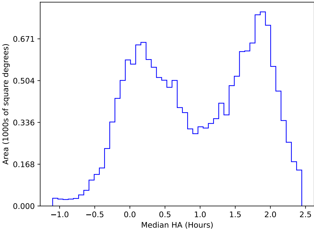
too_elab_r32_d3_gz_v3.4_10yrs WFD u band: Median HA
