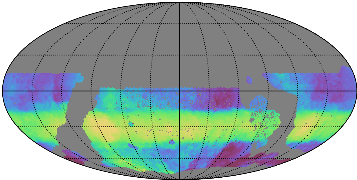
too_elab_r32_d3_gz_v3.4_10yrs WFD r band: Median HA
