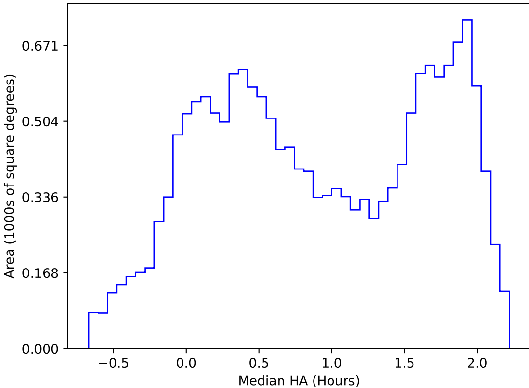
too_elab_r32_d3_gz_v3.4_10yrs WFD r band: Median HA
