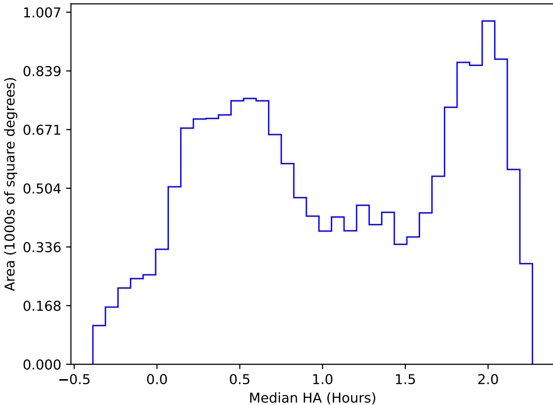
too_elab_r32_d3_gz_v3.4_10yrs WFD i band: Median HA
