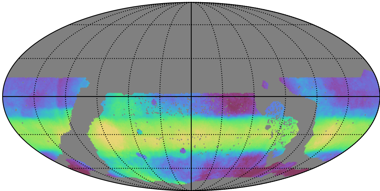
too_elab_r32_d3_gz_v3.4_10yrs WFD all bands: Median HA
