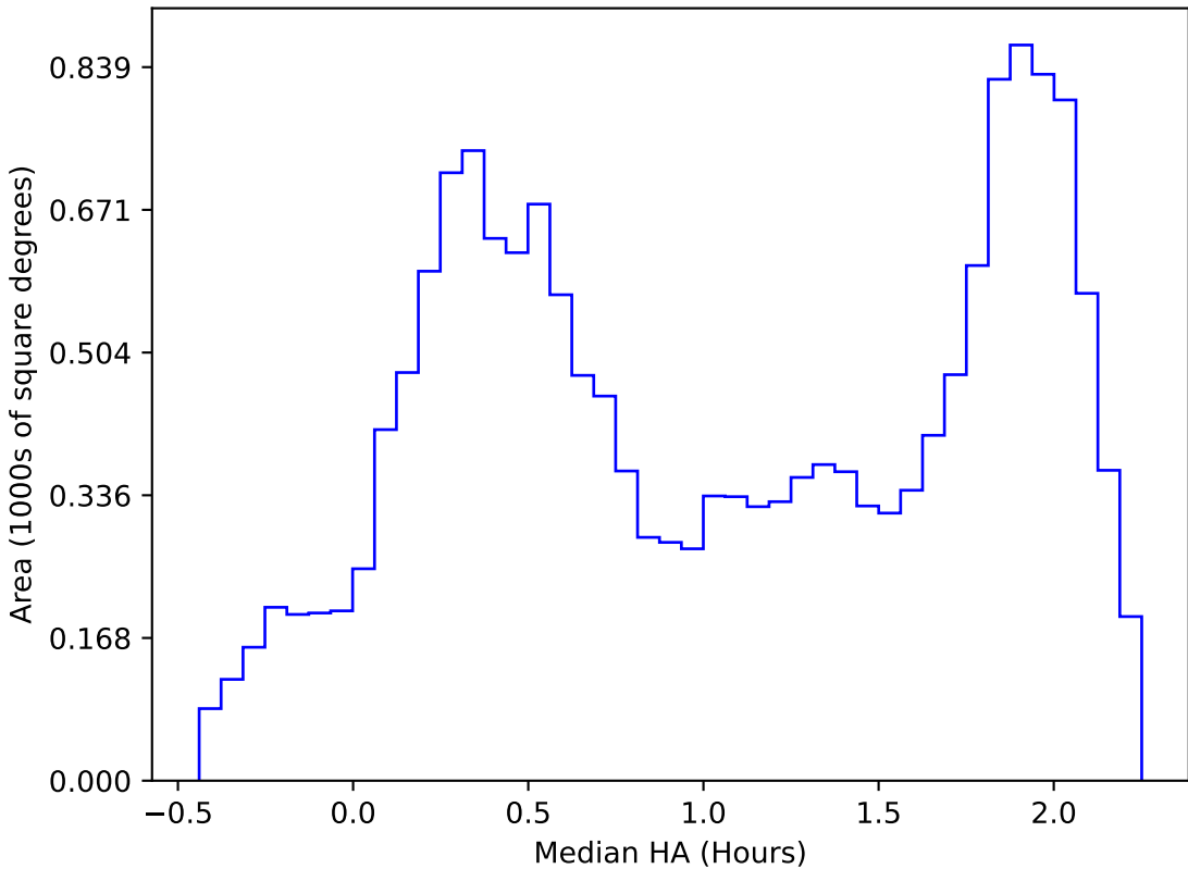
too_elab_r32_d3_gz_v3.4_10yrs WFD all bands: Median HA
