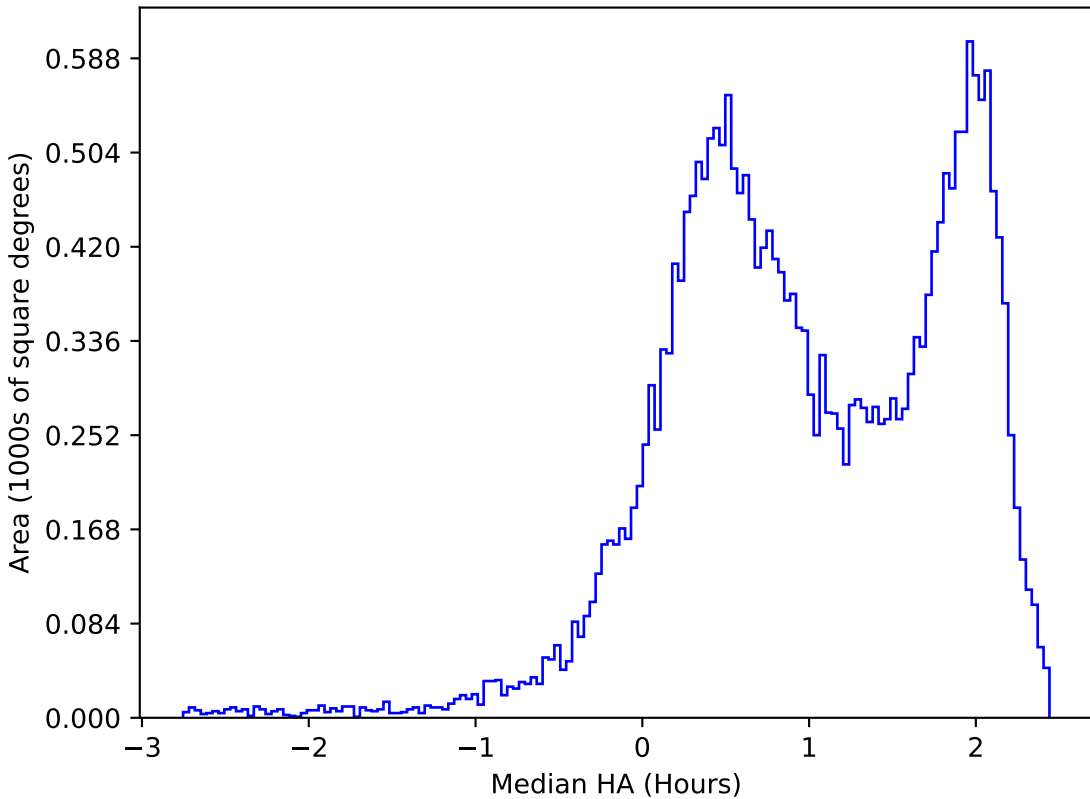
too_elab_r32_d3_gz_v3.4_10yrs All sky z band: Median HA
