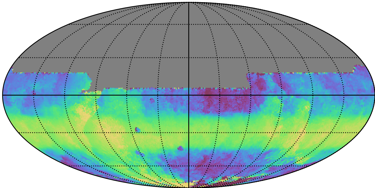
too_elab_r32_d3_gz_v3.4_10yrs All sky y band: Median HA
