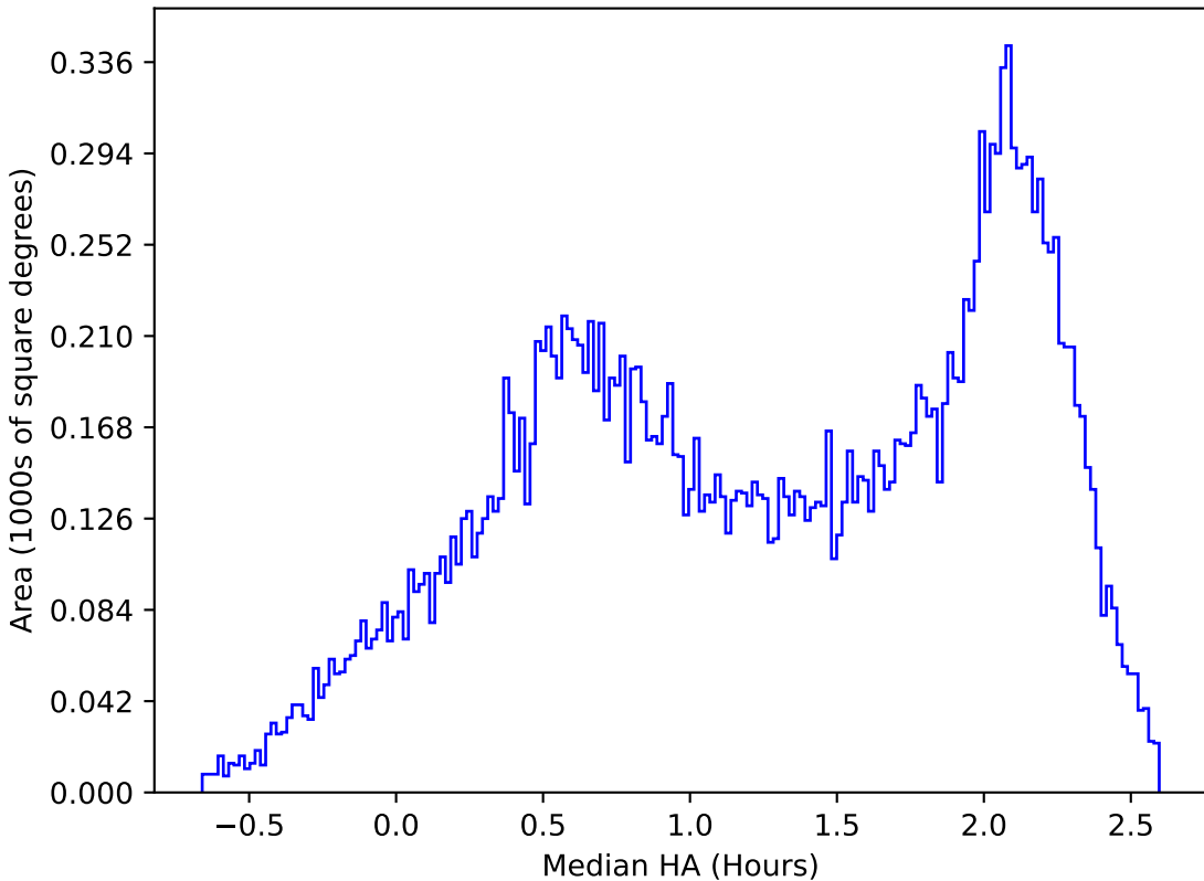
too_elab_r32_d3_gz_v3.4_10yrs All sky y band: Median HA
