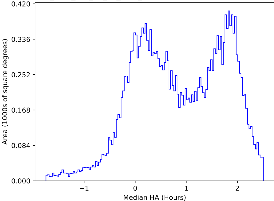
too_elab_r32_d3_gz_v3.4_10yrs All sky u band: Median HA
