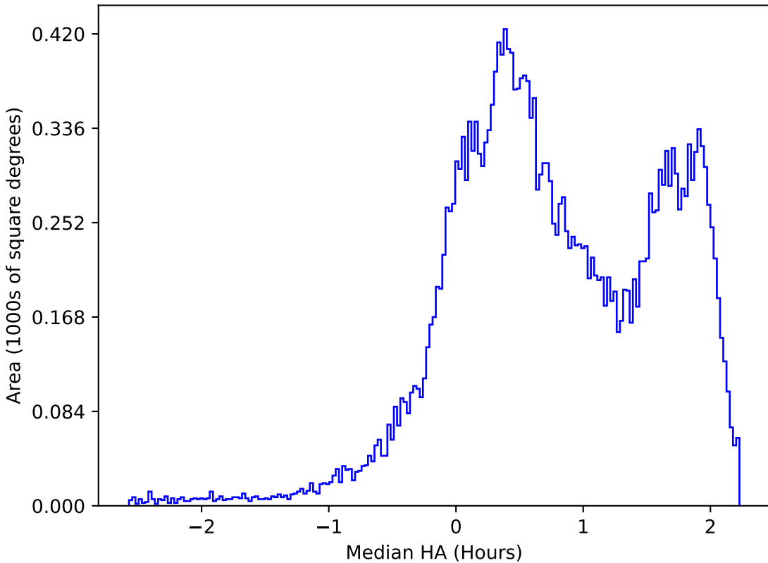
too_elab_r32_d3_gz_v3.4_10yrs All sky r band: Median HA
