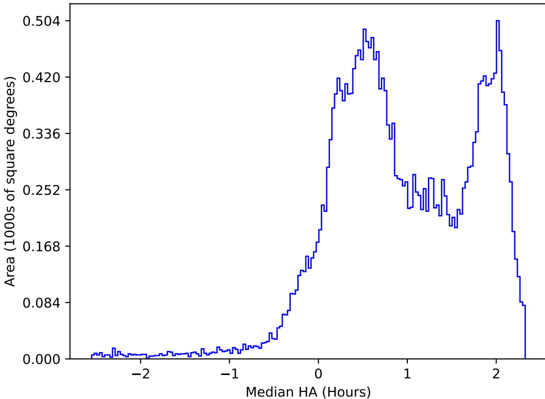
too_elab_r32_d3_gz_v3.4_10yrs All sky i band: Median HA
