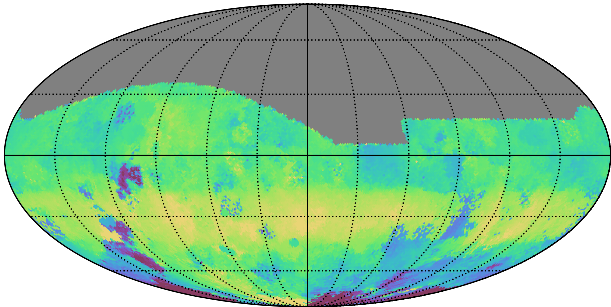
too_elab_r32_d3_gz_v3.4_10yrs All sky g band: Median HA
