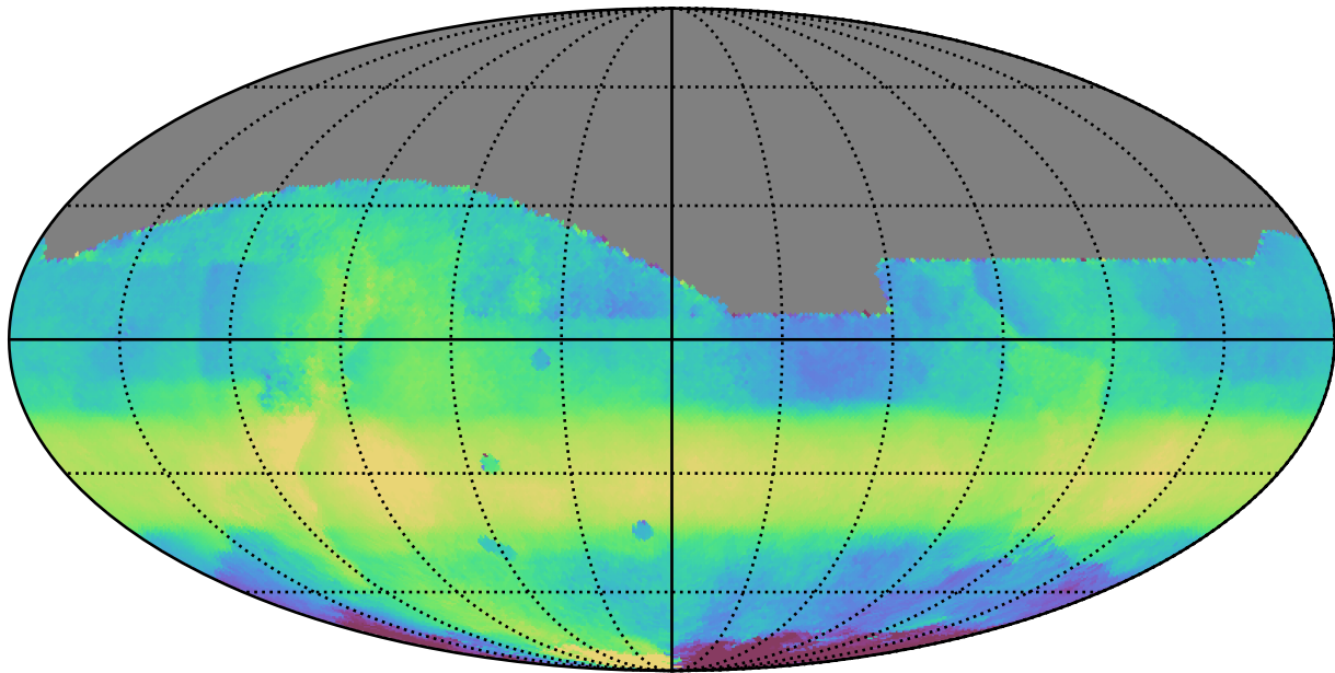
too_elab_r32_d3_gz_v3.4_10yrs All sky all bands: Median HA
