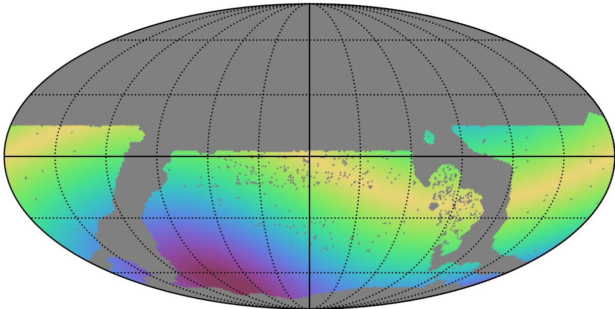
too_elab_r32_d3_gz_v3.4_10yrs WFD z band: Max solarElong
