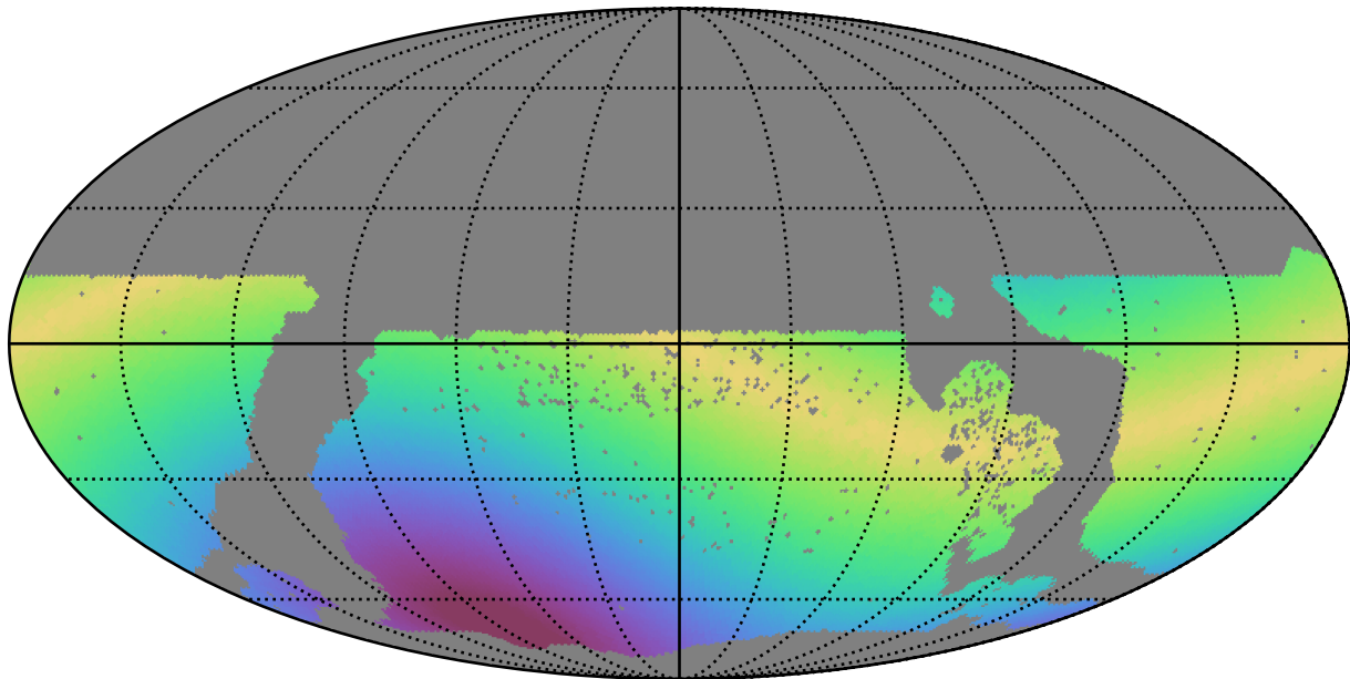
too_elab_r32_d3_gz_v3.4_10yrs WFD y band: Max solarElong
