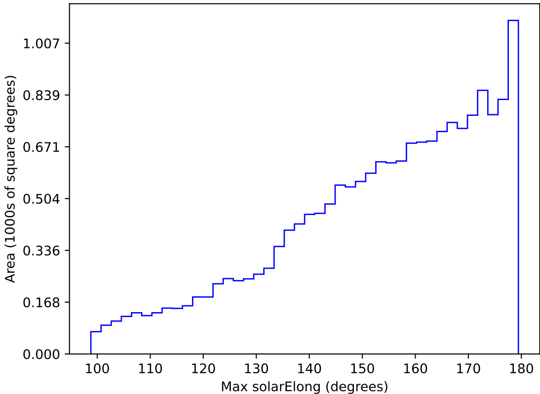
too_elab_r32_d3_gz_v3.4_10yrs WFD r band: Max solarElong
