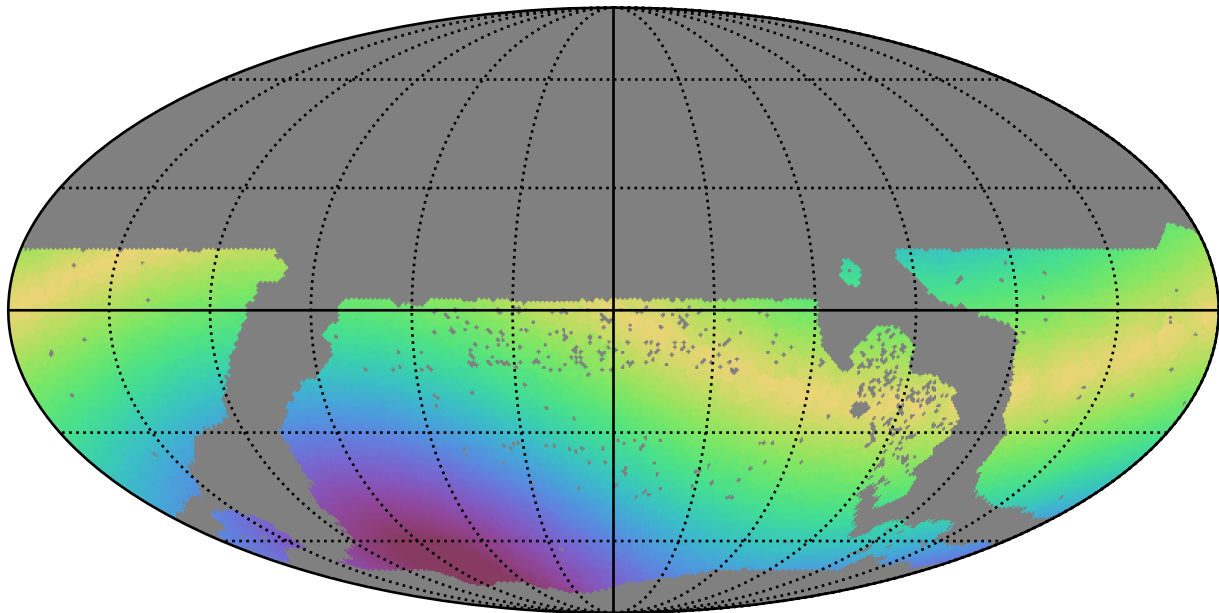
too_elab_r32_d3_gz_v3.4_10yrs WFD g band: Max solarElong
