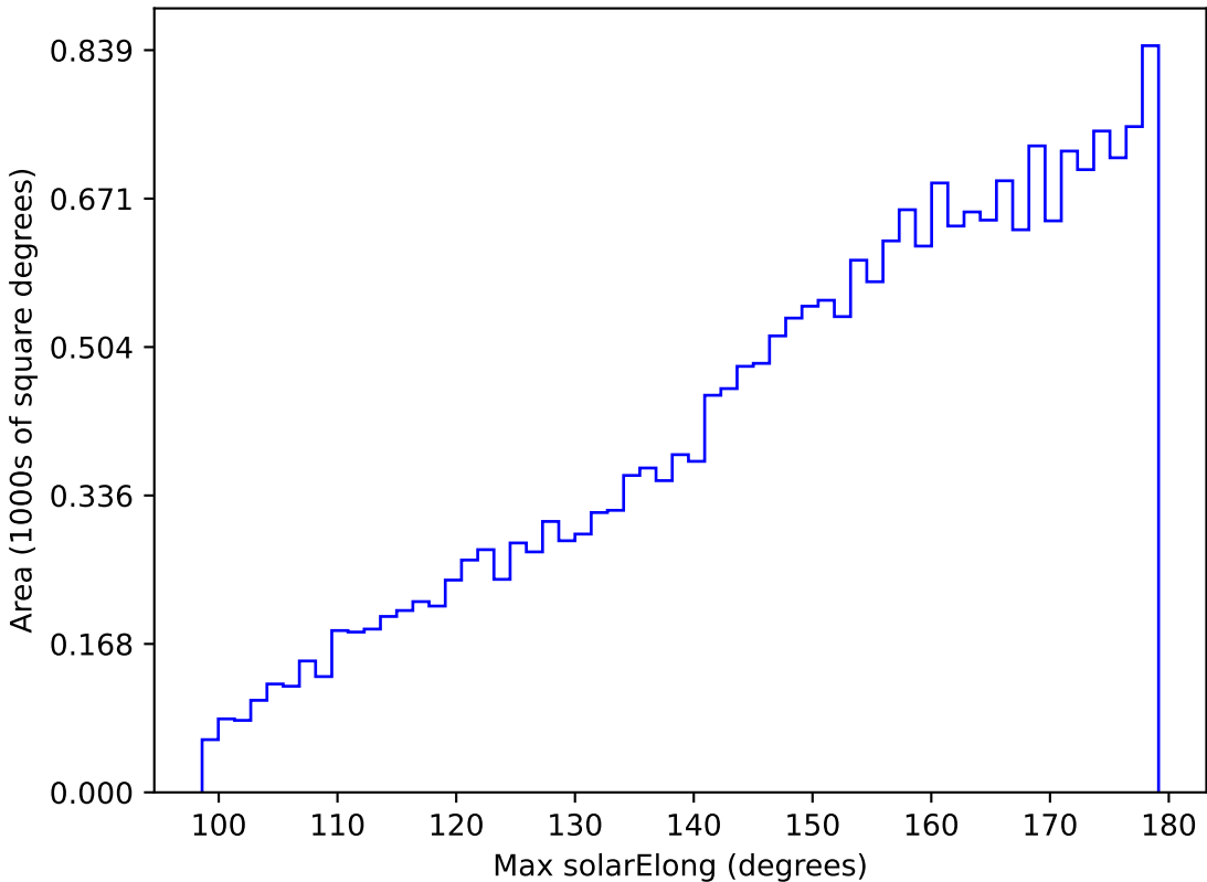
too_elab_r32_d3_gz_v3.4_10yrs All sky y band: Max solarElong
