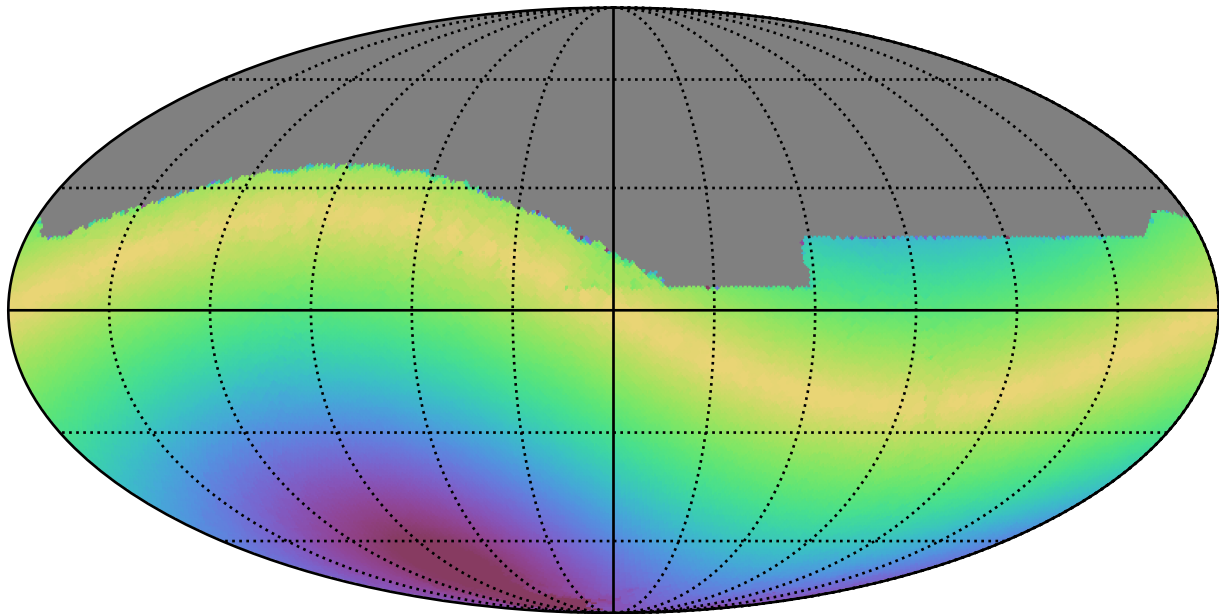
too_elab_r32_d3_gz_v3.4_10yrs All sky r band: Max solarElong
