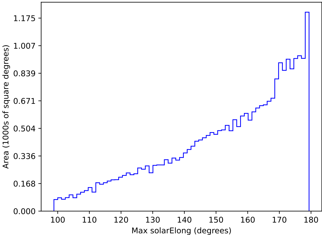
too_elab_r32_d3_gz_v3.4_10yrs All sky r band: Max solarElong
