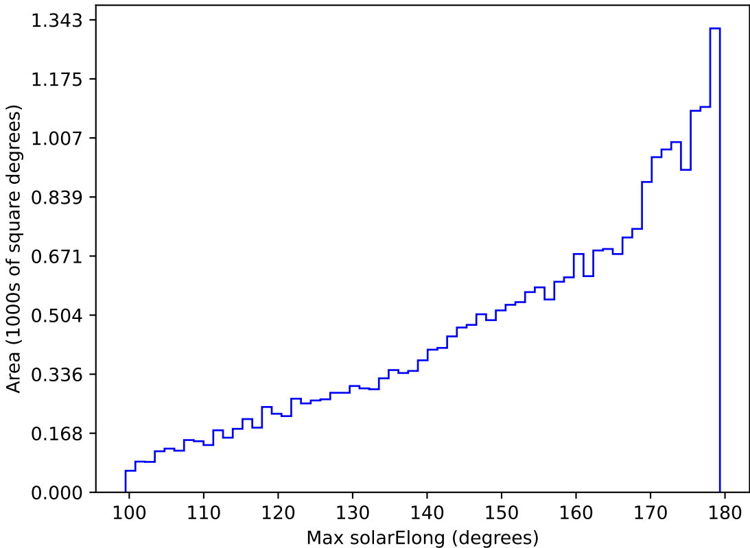
too_elab_r32_d3_gz_v3.4_10yrs All sky i band: Max solarElong
