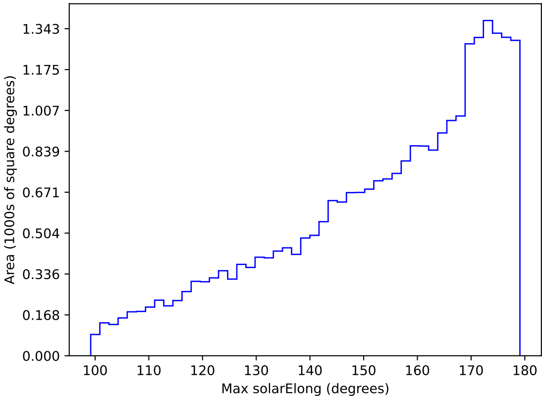
too_elab_r32_d3_gz_v3.4_10yrs All sky g band: Max solarElong
