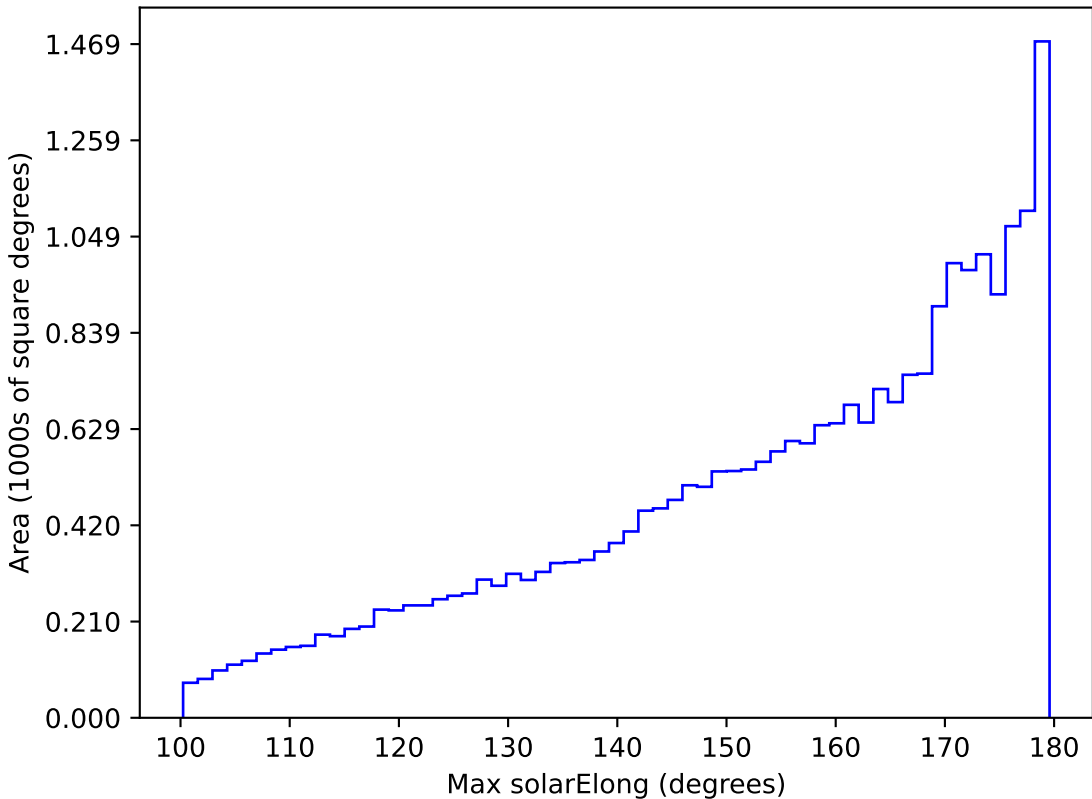
too_elab_r32_d3_gz_v3.4_10yrs All sky all bands: Max solarElong
