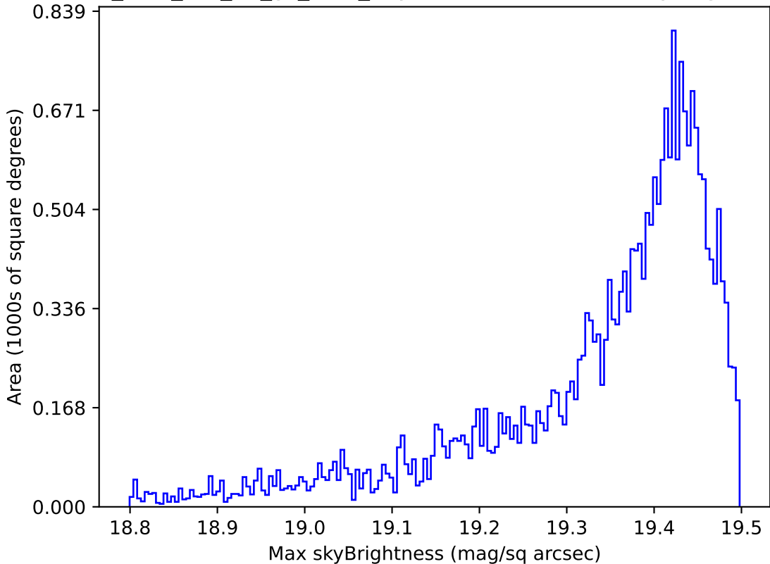
too_elab_r32_d3_gz_v3.4_10yrs Yr 1 z band: Max skyBrightness
