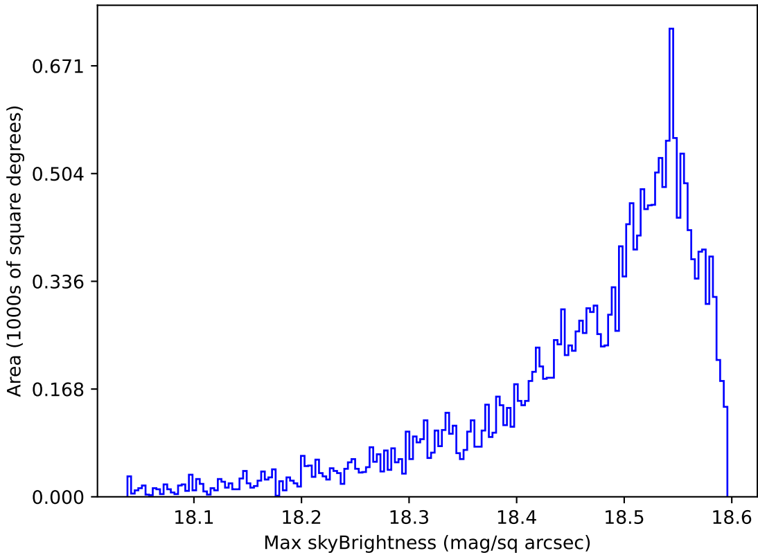
too_elab_r32_d3_gz_v3.4_10yrs Yr 1 y band: Max skyBrightness
