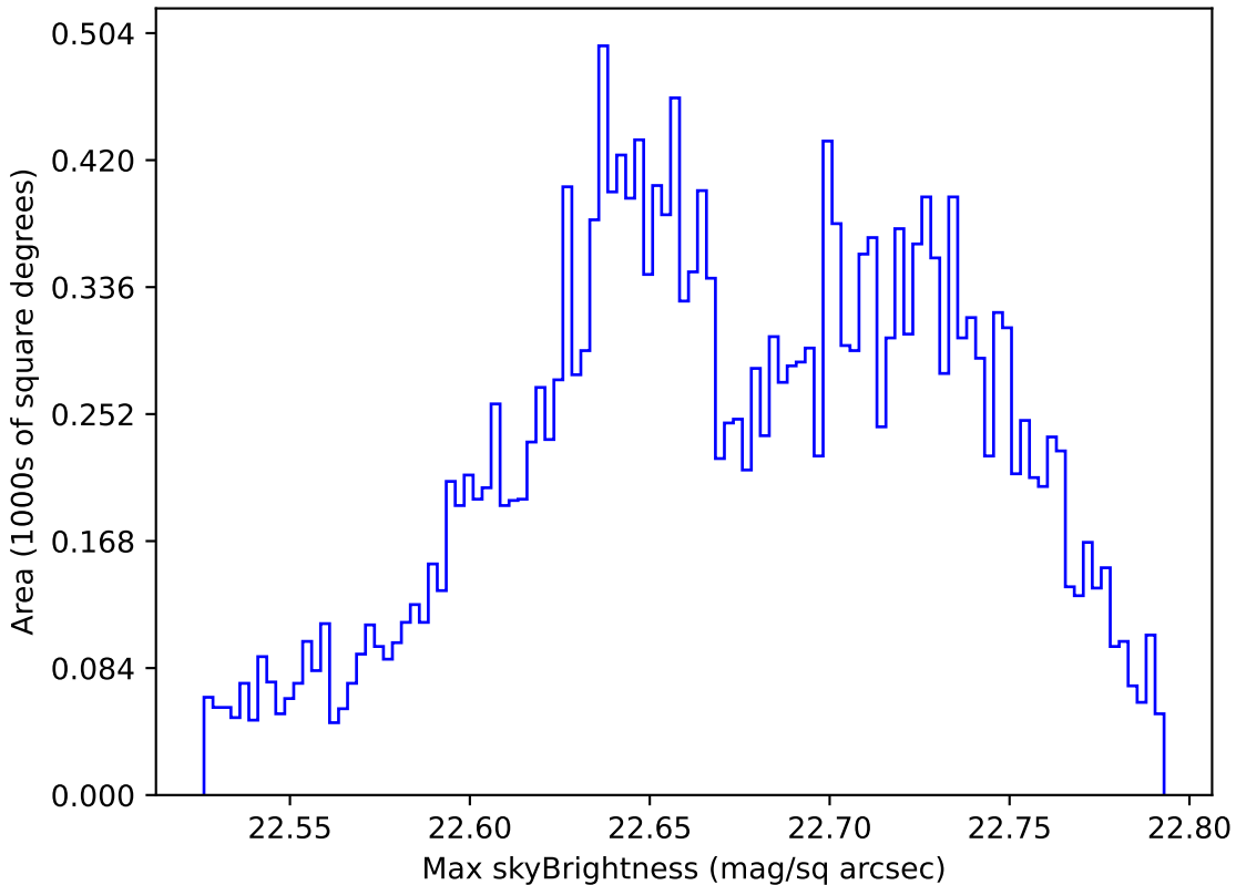
too_elab_r32_d3_gz_v3.4_10yrs Yr 1 u band: Max skyBrightness
