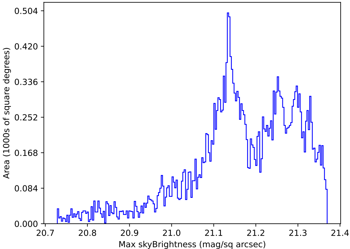
too_elab_r32_d3_gz_v3.4_10yrs Yr 1 r band: Max skyBrightness
