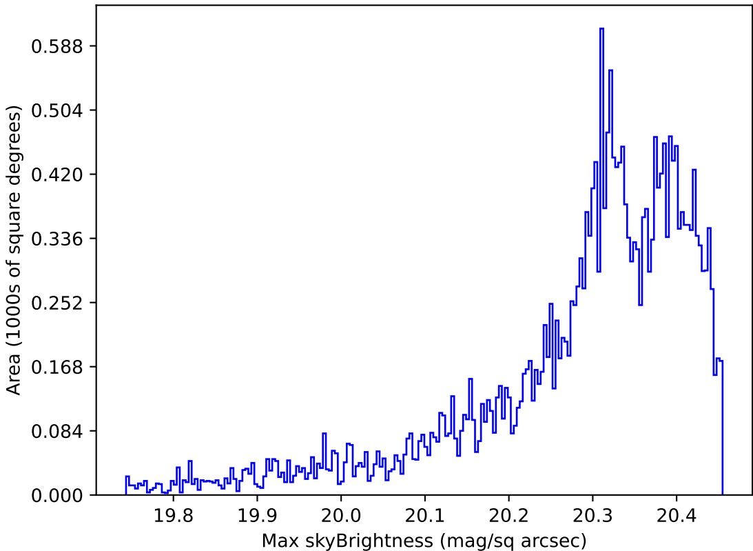
too_elab_r32_d3_gz_v3.4_10yrs Yr 1 i band: Max skyBrightness
