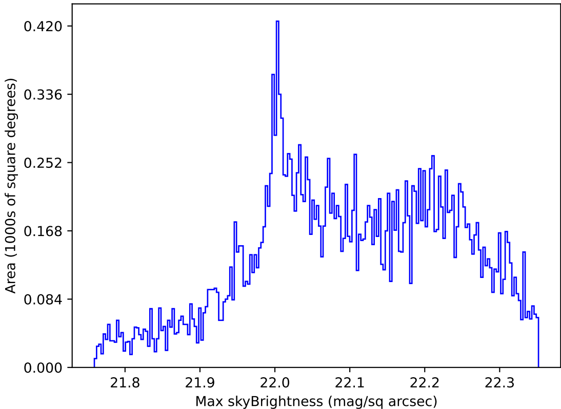
too_elab_r32_d3_gz_v3.4_10yrs Yr 1 g band: Max skyBrightness
