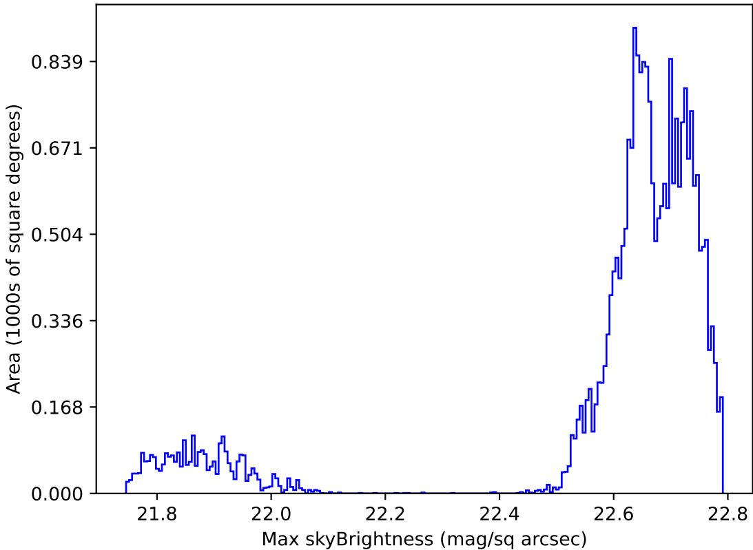
too_elab_r32_d3_gz_v3.4_10yrs Yr 1 all bands: Max skyBrightness
